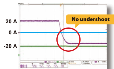
DC SEAM mode operation example
