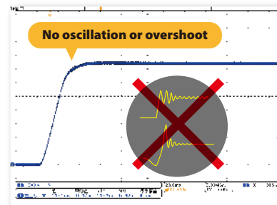
Output voltage waveform with 400 µF capacitor connected
